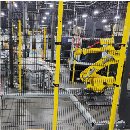
ROBOTIC GUARDING
