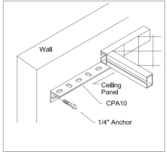
CPA10 to Wall
