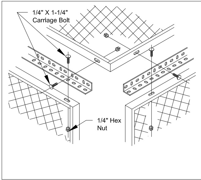
CPA10 Base Panel to Ceiling Panel
