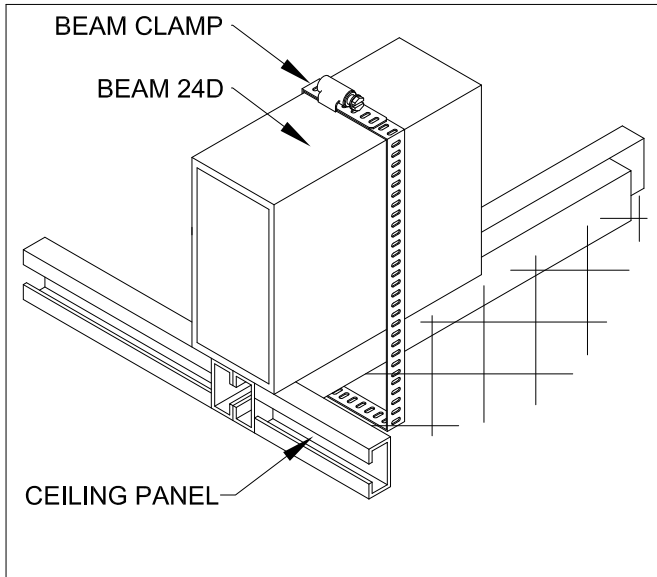
BEAM24 Assembly
