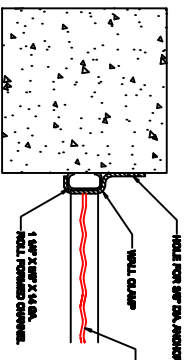
WALL CLAMP CONNECTION
