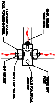
THREE WAY POST
